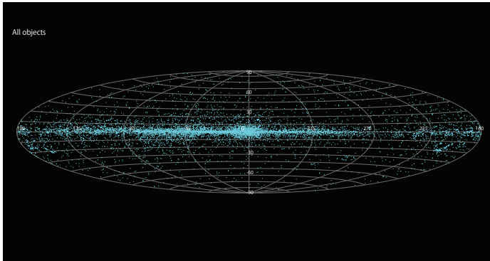
Figure 1. Distribution in Galactic coordinates of > 10000 objects included in the eDAMS database. These objects are observed, at least, in one of the OH, H 2 O and SiO maser lines, and the both detections and non-detections are included.
